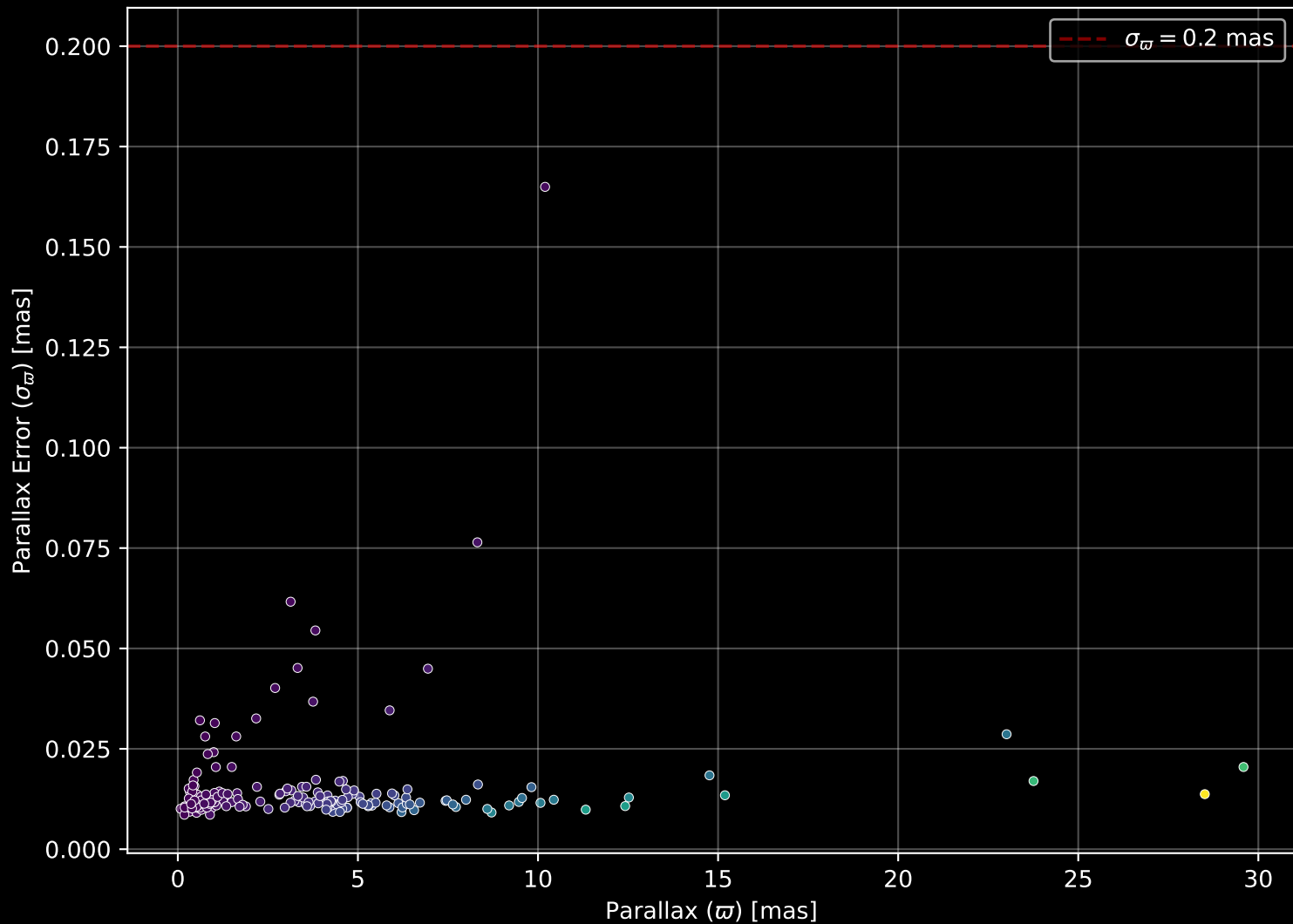
APOGEE DR17 Field: [CVZTILE_105+36_btx] Parallax Quality (n= 191)
