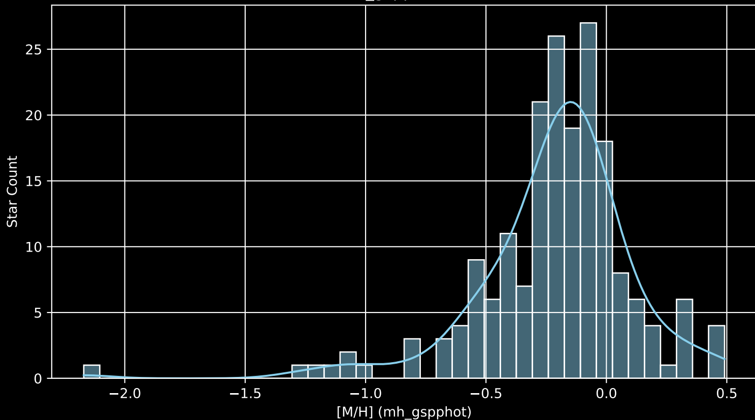
APOGEE DR17 Field: [CVZTILE_105+36_btx [M/H] (mh_gspphot) (n= 190)
