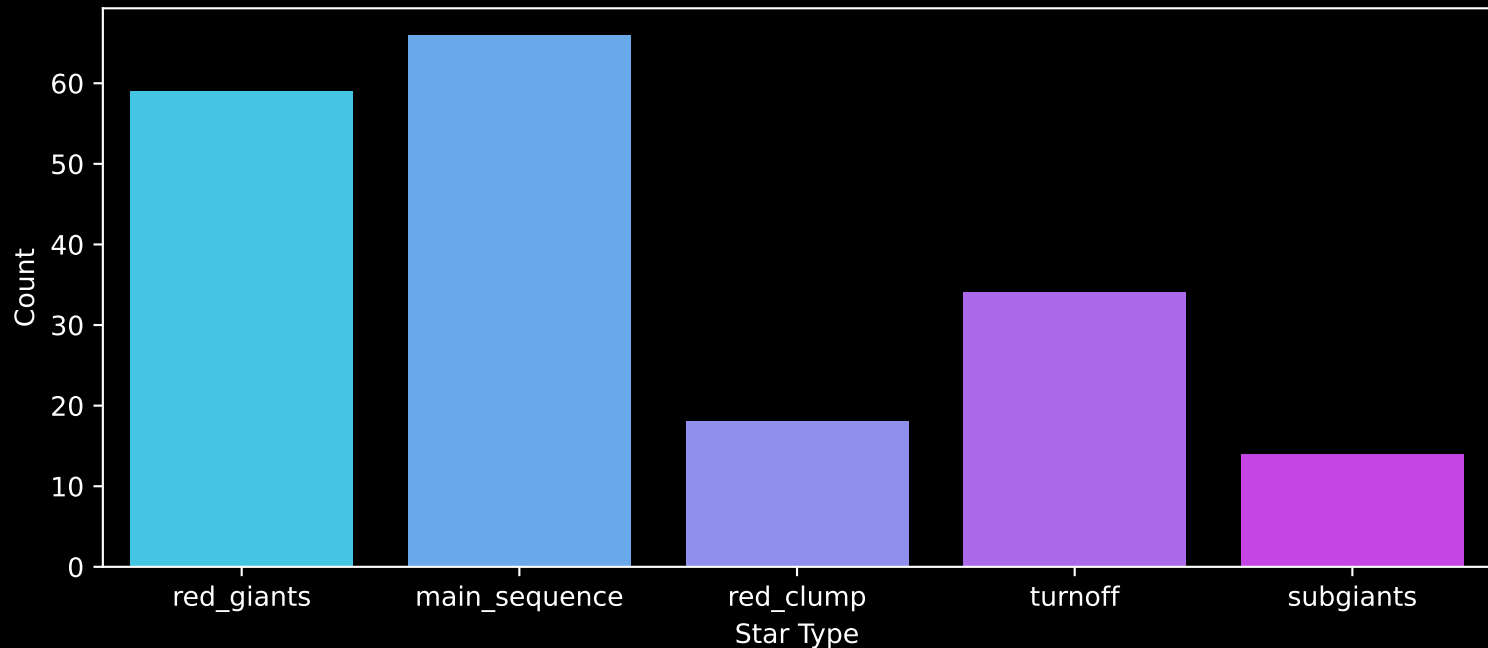
APOGEE DR17 Field: [CVZTILE_105+36_btx] Count plot of Star Type
