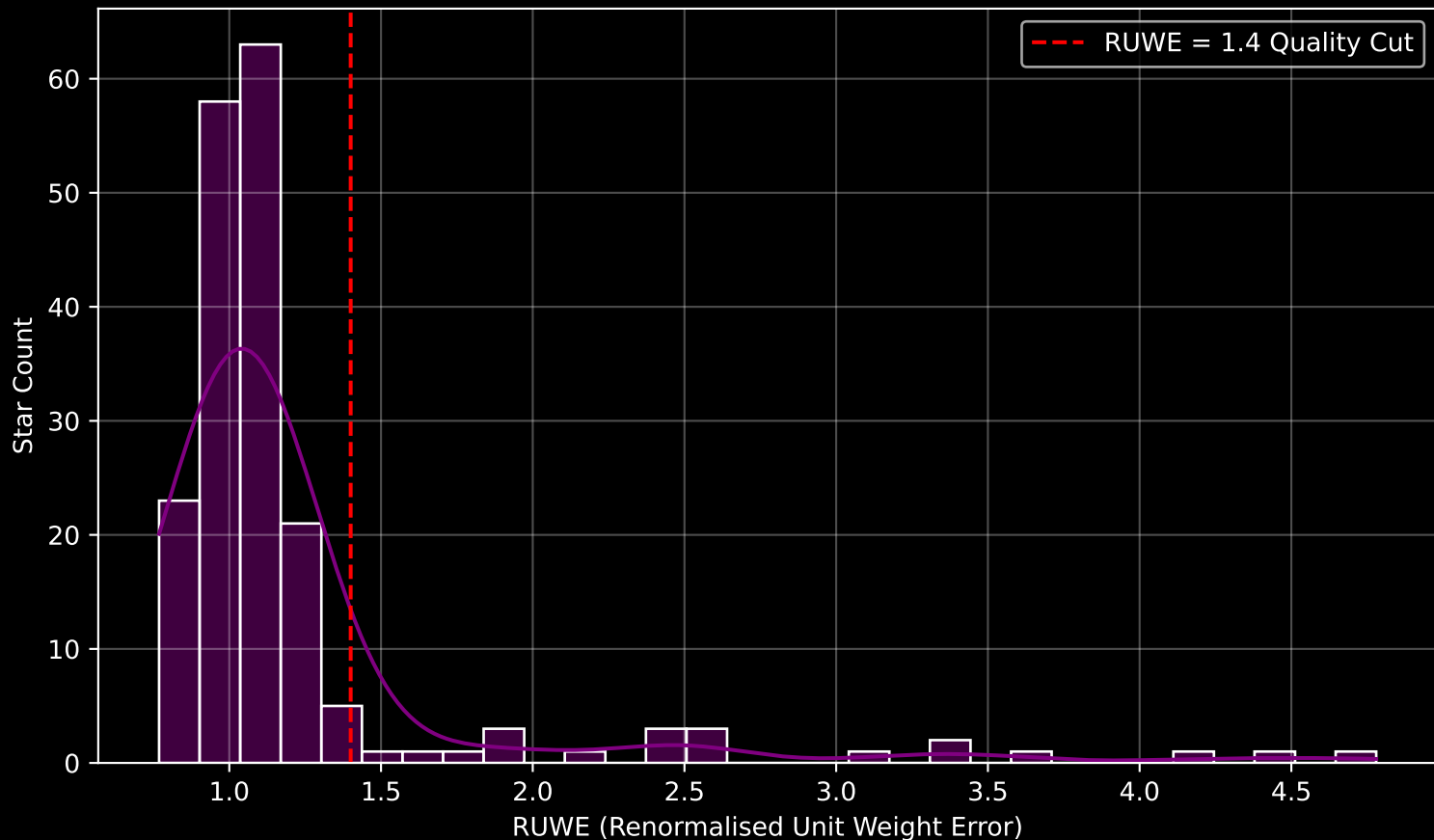
GAPOGEE DR17 Field [CVZTILE_105+36_btx] RUWE Distribution (n= 190)
