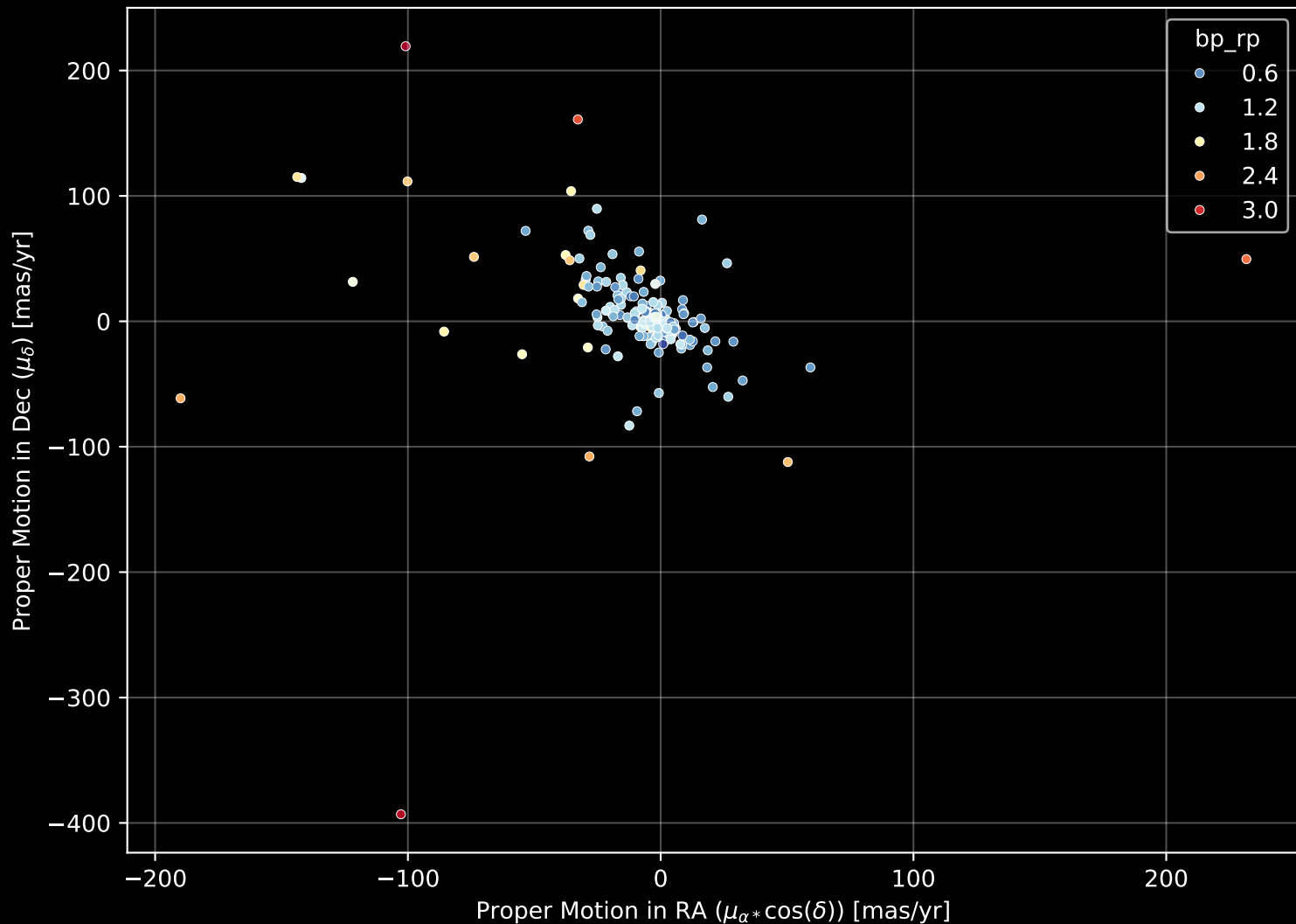
APOGEE DR17 Field: [CVZTILE_105+36_btx] Proper Motion Diagram (n= 191)
