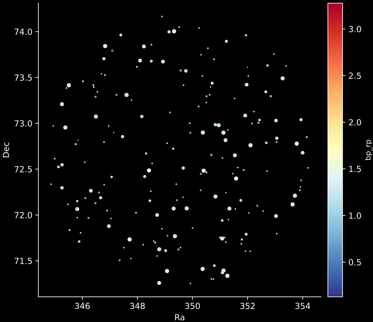
APOGEE DR17 Field: [CVZTILE_105+36_btx] Stars: 191
